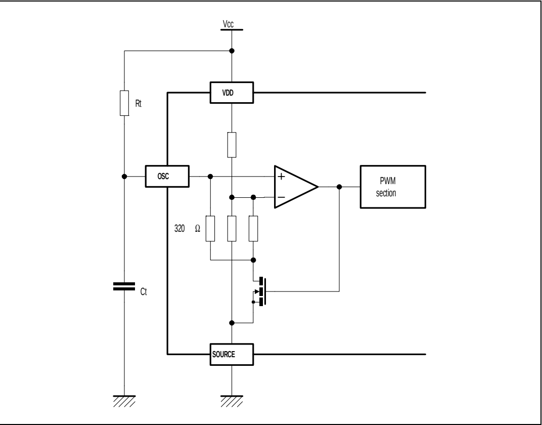
Figure 15. Oscillator Schematic
