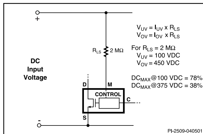
Figure 31. Line-Sensing for Undervoltage, Overvoltage and Line Feed-Forward.
