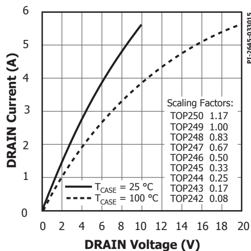
Figure 67. Output Characteristics.
