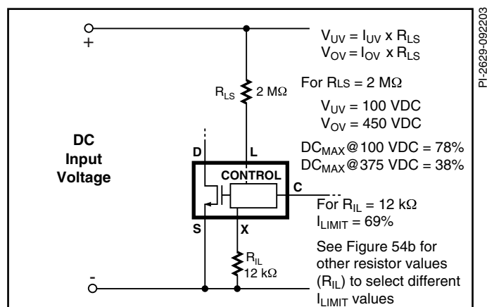
Figure 28. Line-Sensing and Externally Set Current Limit.
