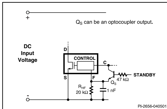
Figure 15. Half Frequency Standby Mode (For High Standby Efficiency).
