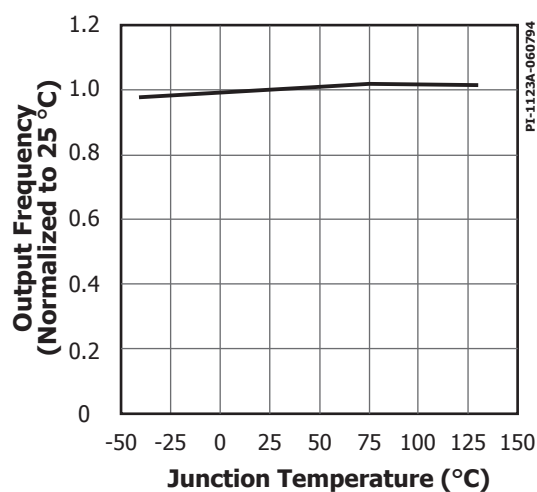
Figure 58. Frequency vs. Temperature.
