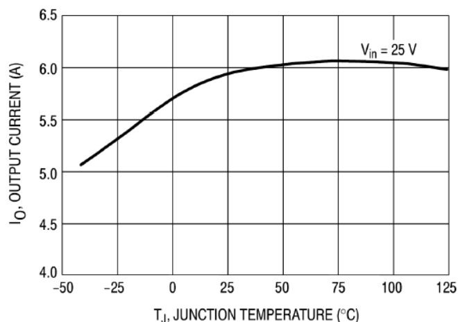
Figure 5. Current Limit
