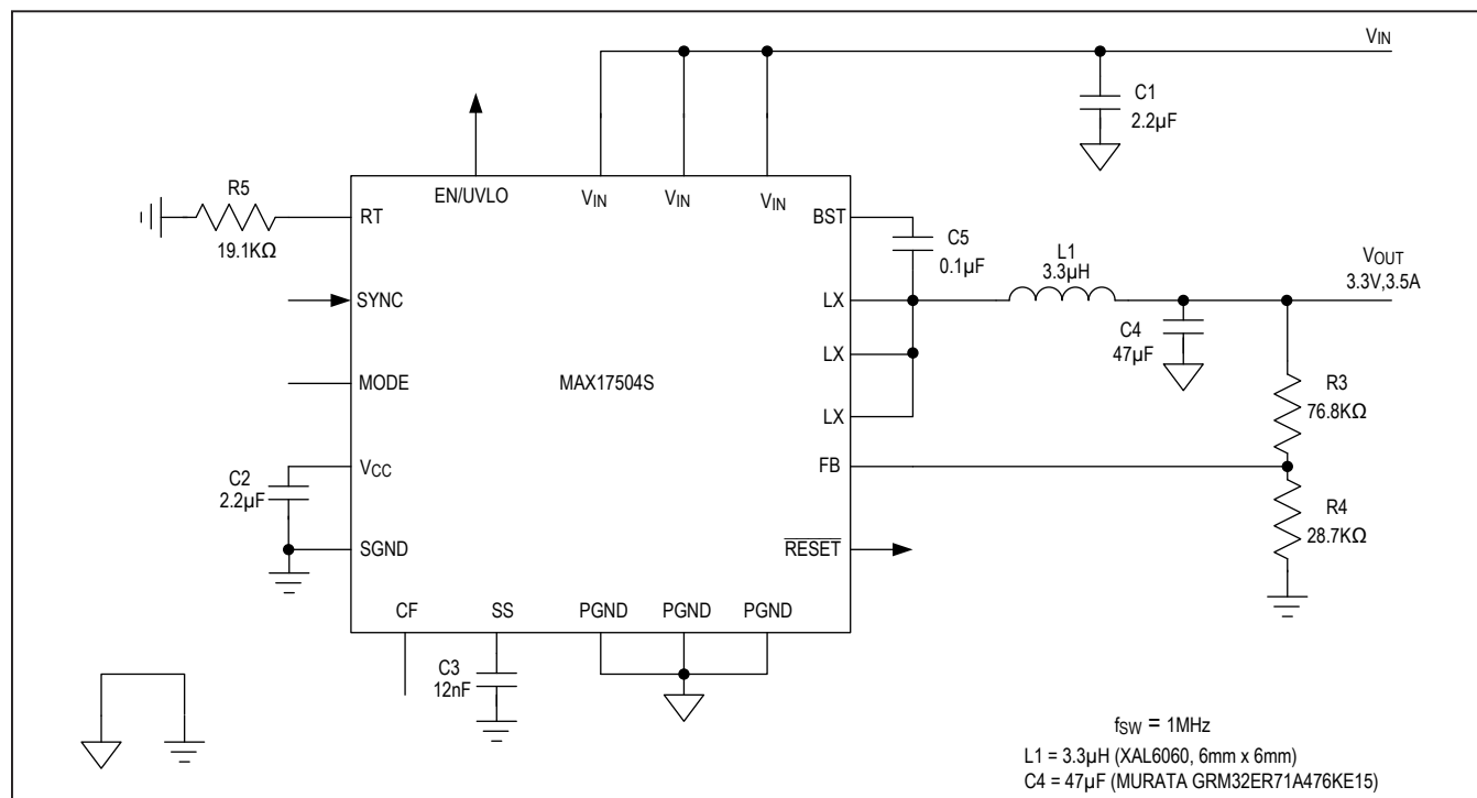
Figure 6. MAX17504S Typical Operating Circuit for 3.3V Output, 1MHz Switching Frequency
