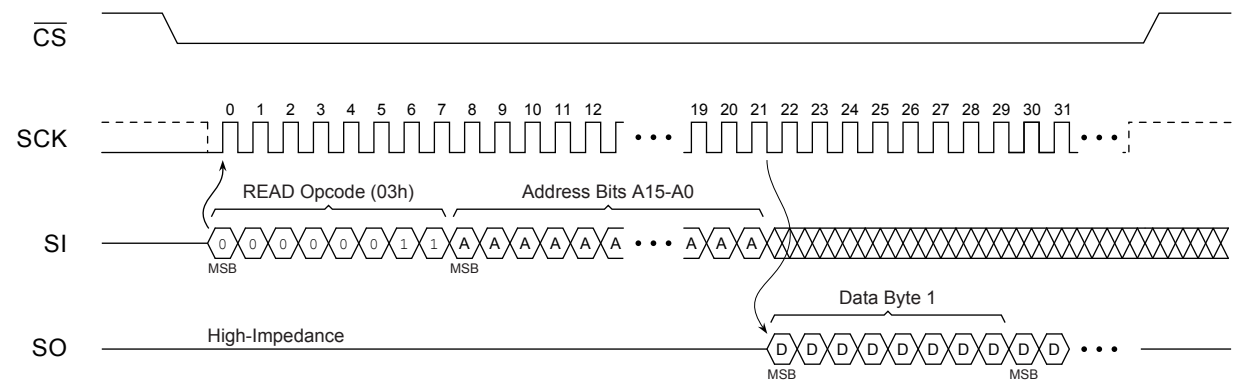
Figure 7-1. Read Waveform
