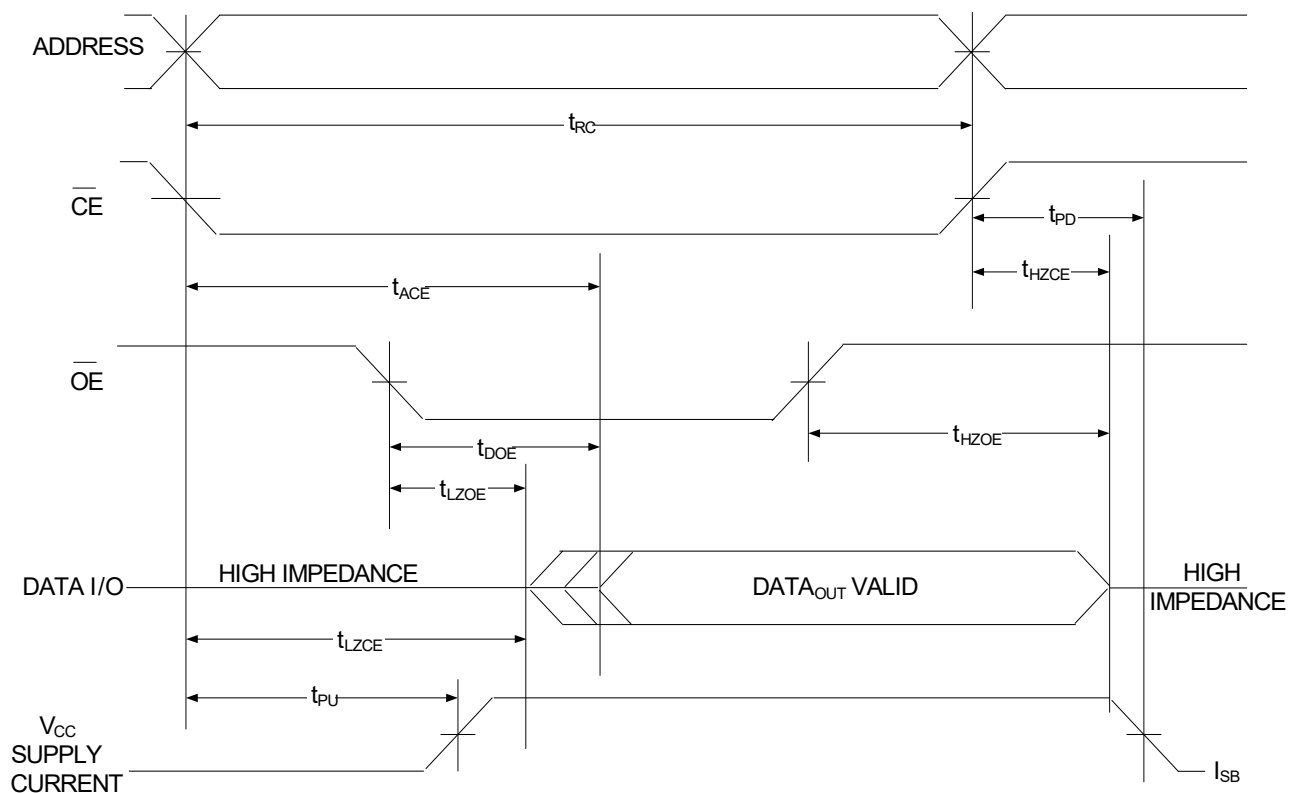
Figure 6. Read Cycle No. 2 ( \overline{\text{OE}} Controlled) [15, 16]
