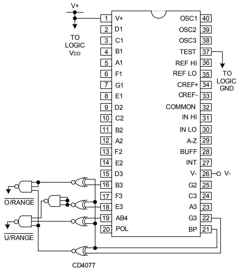
Figure 10. Circuit for Developing Underrange and Overrange from UTC 7106 Outputs
