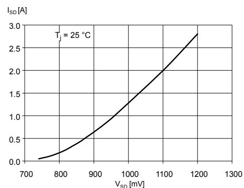
Figure 39. Typical drain-source diode forward ON characteristic
