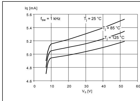
Figure 34. Typical quiescent current vs. supply voltage
