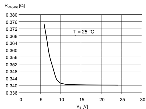
Figure 35. Typical high-side R_{DS(ON)} vs. supply voltage
