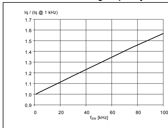
Figure 36. Normalized typical quiescent current vs. switching frequency
