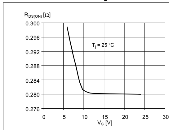
Figure 38. Typical low-side R_{DS(ON)} vs. supply voltage
