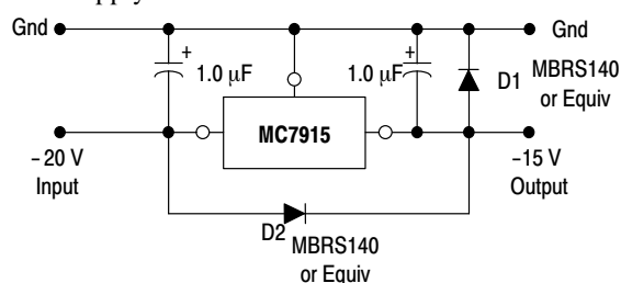
Figure 11. Protection Diodes
