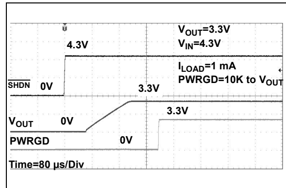
FIGURE 2-28: Start-up from SHDN.
