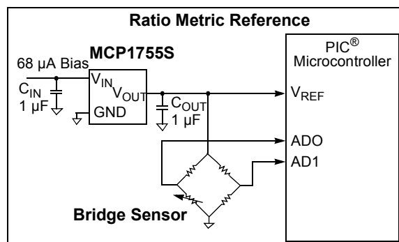
FIGURE 5-2: Using the MCP1755/1755S as a Voltage Reference.
