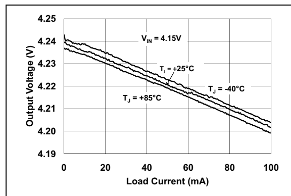
FIGURE 2-6: Output Voltage vs. Load Current ( V_R = 4.2\text{V} ).
