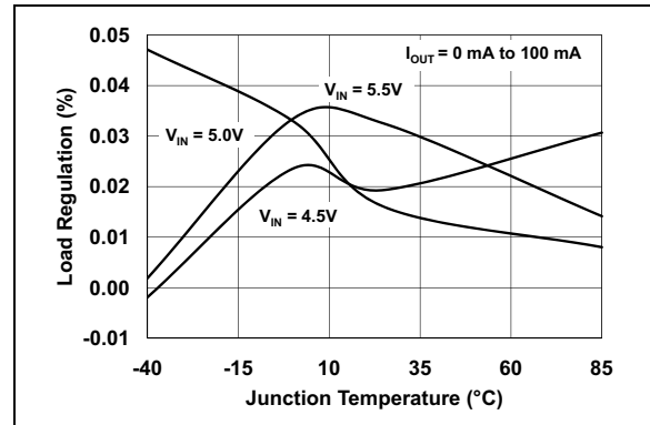
FIGURE 2-27: Load Regulation vs. Junction Temperature ( V_R = 4.2\text{V} ).
