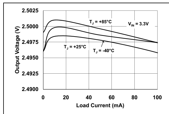
FIGURE 2-5: Output Voltage vs. Load Current ( V_R = 2.5\text{V} ).
