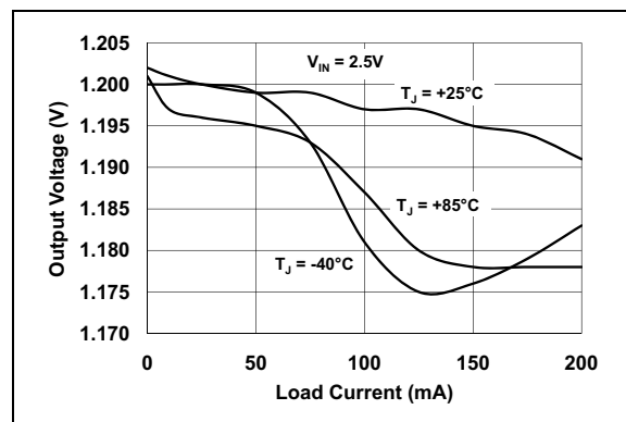
FIGURE 2-4: Output Voltage vs. Load Current ( V_R = 1.2\text{V} ).
